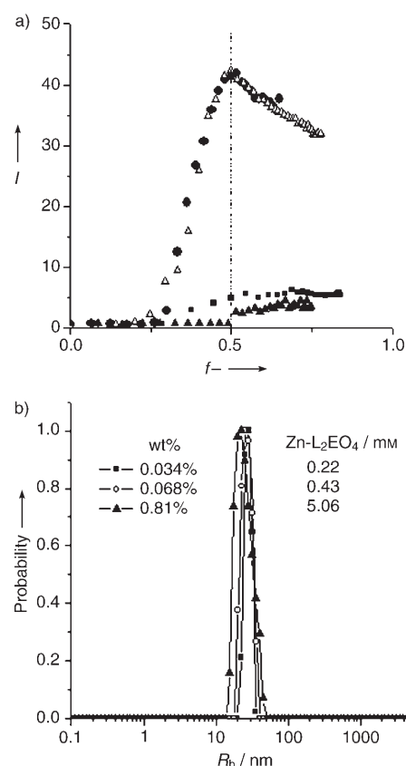
Figure 1. a) Variation of the scattered light intensity I with the mixing fraction f_- , on addition of the Zn-L 2 EO 4 coordination polymer to a solution of PMVP 41 - b -PEO 205 ( \Delta ), L 2 EO 4 to PMVP 41 - b -PEO 205 ( \blacksquare ), L 2 EO 4 to the mixed solution of (Zn 2+ + PMVP 41 - b -PEO 205 ) ( \bullet ), and L 2 EO 4 -Zn-L 2 EO 4 to PMVP 41 - b -PEO 205 ( \blacktriangle ). b) Distribution of the hydrodynamic radius ( R_h ) from dynamic light scattering (DLS) measurements by using CONTIN analysis for the Zn-L 2 EO 4 /PMVP 41 - b -PEO 205 mixture of different concentrations at f_- = 0.5 . Both the total concentration (wt%) and the molar concentration of Zn-L 2 EO 4 are shown. All the experiments were done at 298 \pm 0.1 K.
